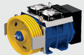
MRL Gearless Machine
