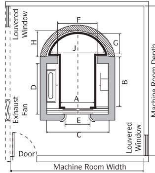
Hoistway Machine Room Plan For Capsule Elevator
